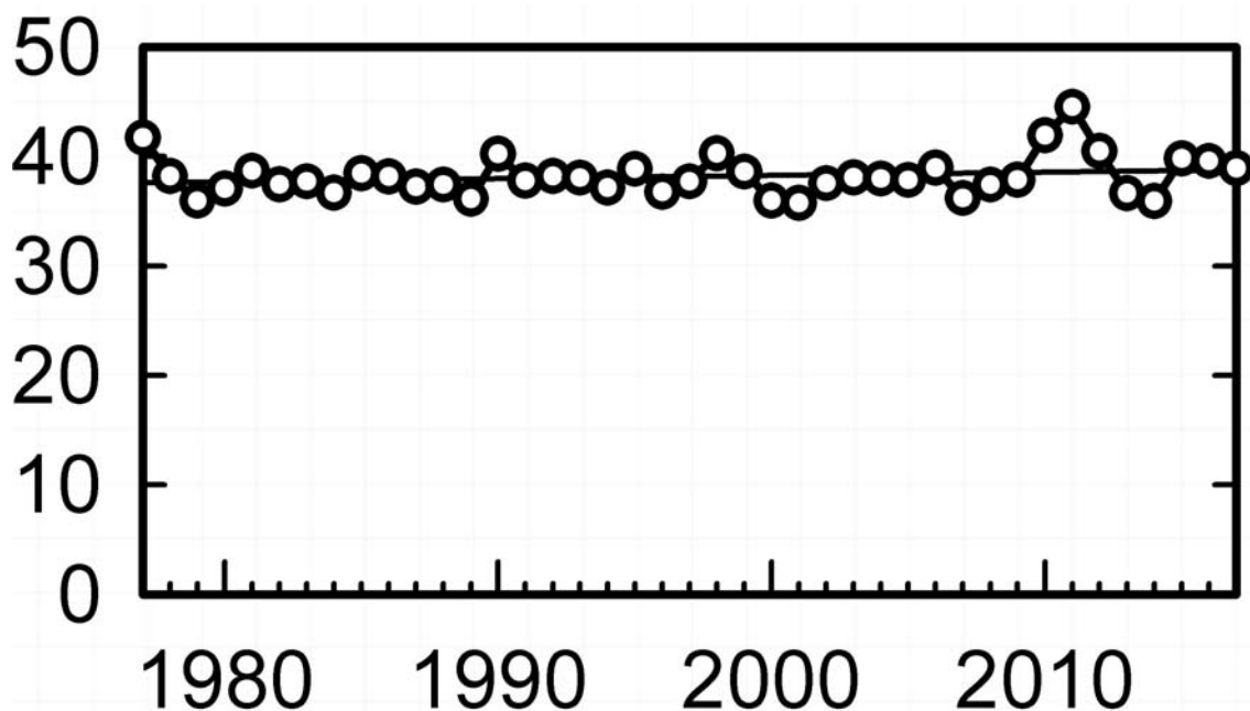
Fig 6: Rugetid (dage) Incubation time (days)
