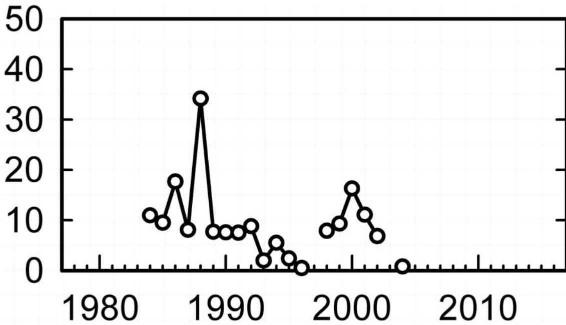
Fig 15: Unge % i oktober i hele fjorden Cygnets % in october in all the fjord
