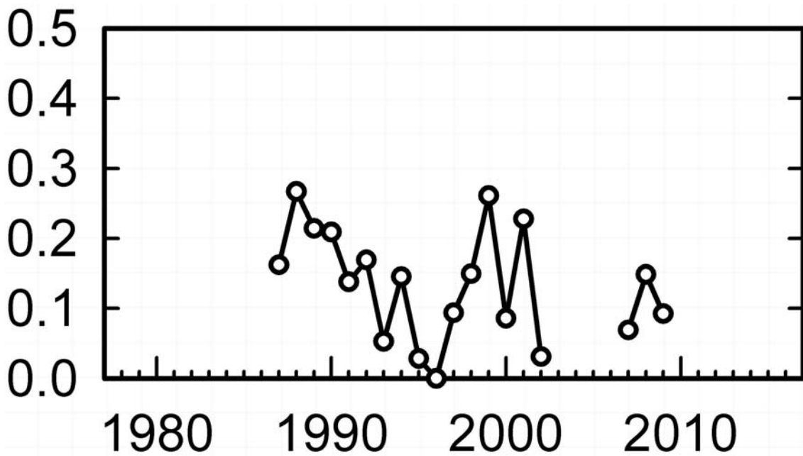
Fig 13: Unger per æg i juli syd for Eskilsø Cygnets per egg in July south of Eskilsø
