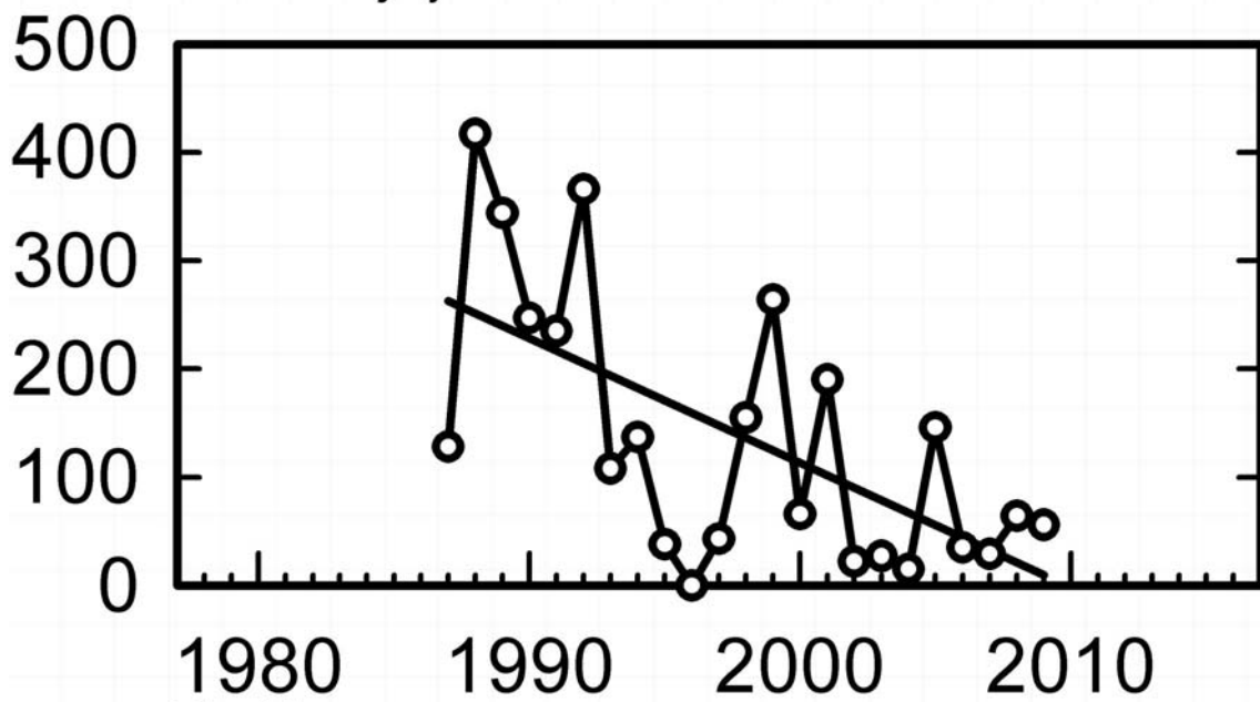
Fig 11: Unger i juli syd for Eskilsø Cygnets in July south of Eskilsø
