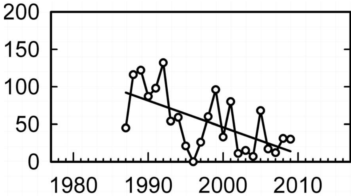
Fig 10: Kuld i juli syd for Eskilsø Broods in July south of Eskilsø
